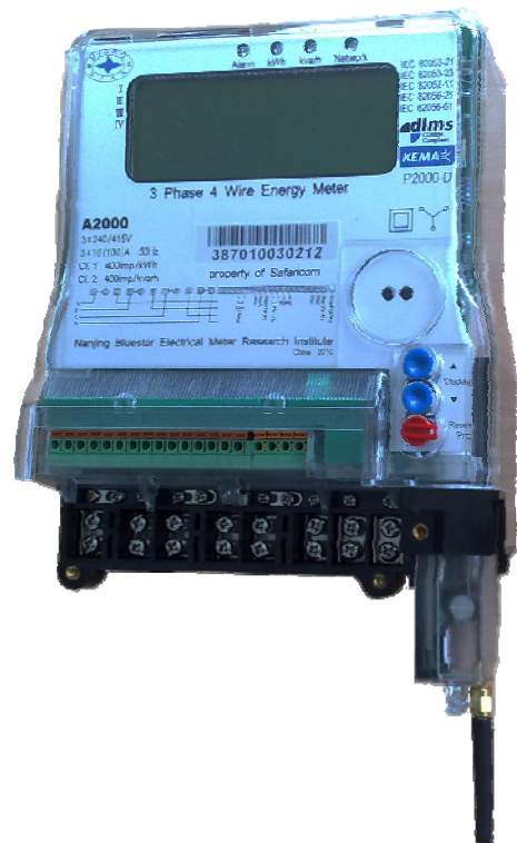
A2000 with Built-in GPRS Modem
